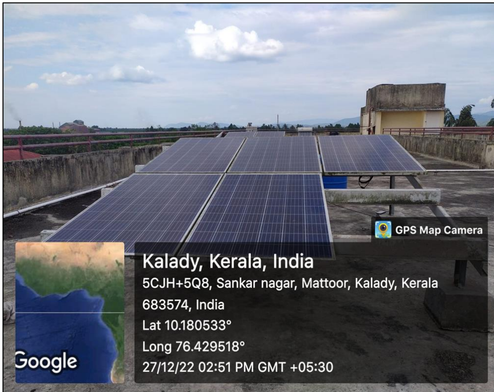
1.5 kW off-grid solar panel is installed by B Voc department, Sree Sankara College
